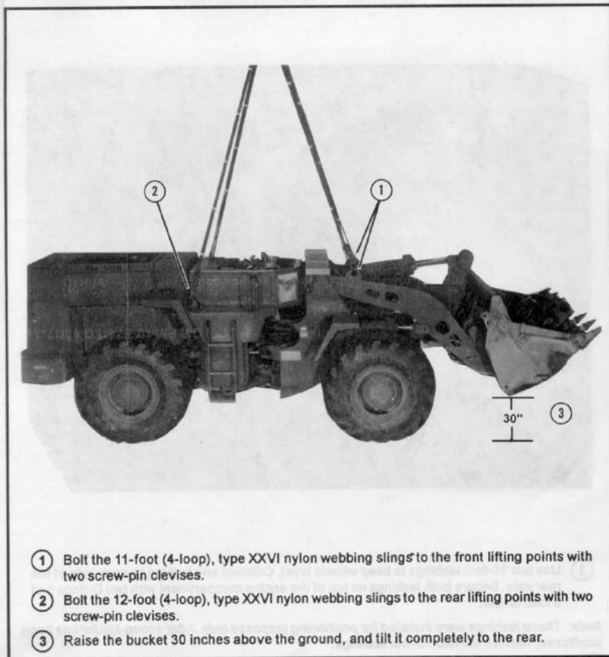
Figure 5-6. Lifting slings installed
