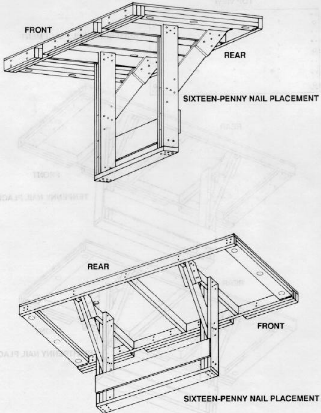
Figure 4-31. Parachute stowage platform built (continued)
